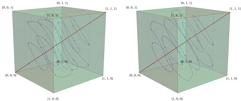
Figure 1. Evolution of the dynamics of FoReL in a 3-player zero-sum polymatrix game with entropic and Euclidean regularization (left and right respectively). The game considered is a graphical variant of Matching Pennies with three players. As can be seen, the trajectories of FoReL orbit the game’s line of Nash equilibria (dark red). The kinks observed in the Euclidean case occur when the support of the trajectory of play changes; by contrast, the multiplicative weights dynamics (left) are interior, so they do not exhibit such kinks.
