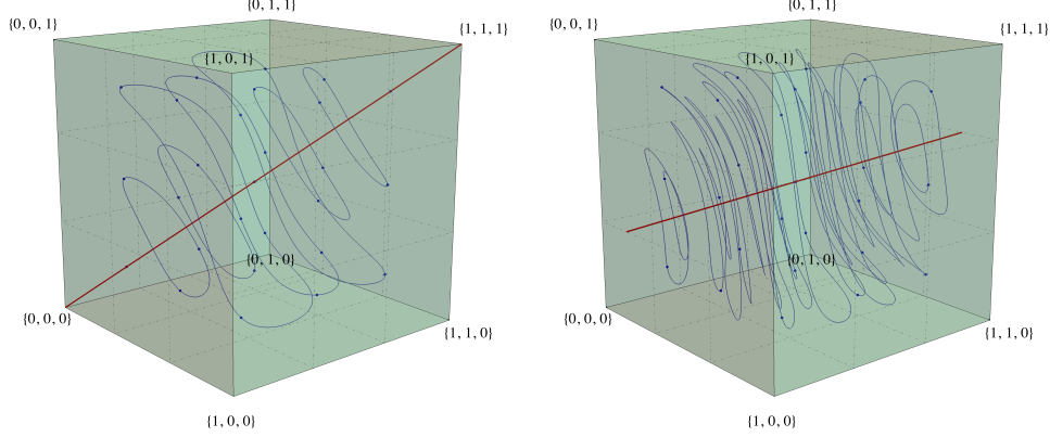
Figure 2. Evolution of the multiplicative weights dynamics (MW) in a 3-player zero-sum polymatrix game. In the left subfigure, each pair of players faces off in a game of standard (symmetric) Matching Pennies; in the right, the game on each pair is weighted by a different factor. In both cases, we plot the solution trajectories of (MW) for the same initial conditions. Even though the different weights change the trajectories of (MW) and the game’s equilibrium set, the cycling behavior of the dynamics remains unaffected.
