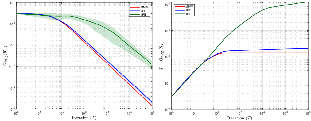
Figure 1: Performance evaluation of the (3MW) with the (2PE) and (1PE) estimators and comparison with the full information (MMW). The solid lines correspond to the mean values of the duality gap of each method, and the shaded regions enclose the area of \pm 1 (sample) standard deviation among the different runs.
