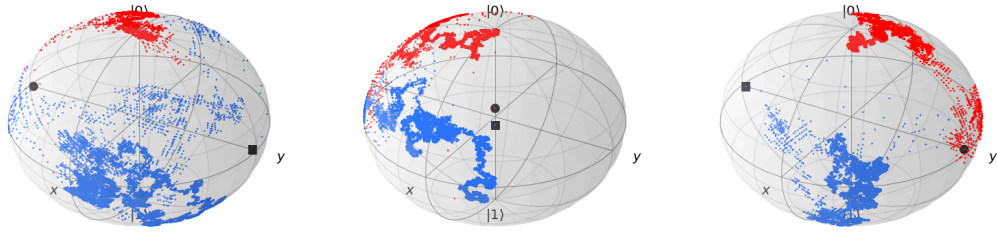
(c) Orbits of (3MW) with bandit feedback as per (1PE)
