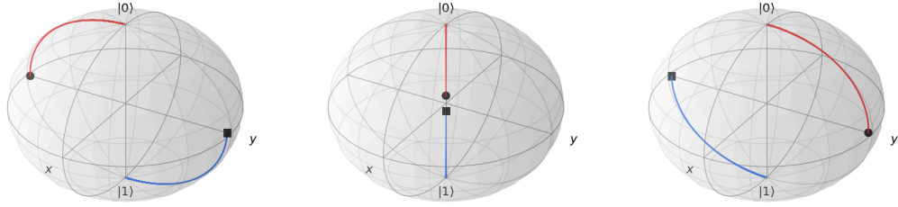
(a) Orbits of (MMW) with full gradient feedback.
