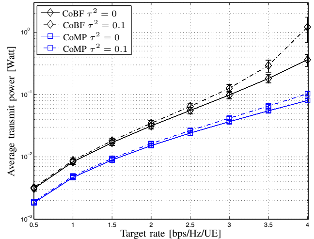
Fig. 2. Average transmit power in Watt vs. target rate when L = 16 , K = 8 and N = 32 .
