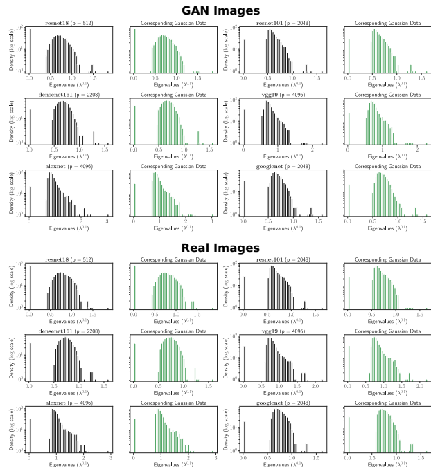
Figure 5. Spectrum of the Gram matrix for CNN representations in (black) and the corresponding Gaussian data (in green) for GAN generated images using the BigGAN model (Brock et al., 2018) (Top) and for real images randomly selected from the Imagenet dataset (Deng et al., 2009) (Bottom). The considered representation network are resnet18 , resnet101 , densenet161 , vgg19 , alexnet and googlenet . We used n = 600 images selected among k = 6 classes {hamburger, mushroom, pizza, strawberry, coffee, daisy} (100 images per class).
