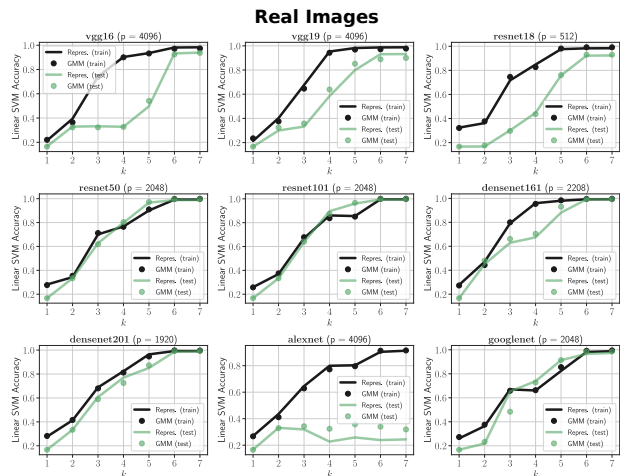
Figure 7. Train and test accuracy of a linear SVM model trained on the top k eigenvectors of the Gram matrix, computed on the representations of Real images. We randomly sampled n = 6000 images belonging to the 6 classes {hamburger, mushroom, pizza, strawberry, coffee, daisy} (1000 images per class) of the Imagenet dataset (Deng et al., 2009). We considered 9 representation networks vgg16 , vgg19 , resnet18 , resnet50 , resnet101 , densenet161 , densenet201 , alexnet and googlenet . Lines represent the performance of the SVM model on the representations themselves whereas dots represent the performance of the SVM model on Gaussian data with the same first and second order moments. We used a train vs test split of 2/3 and 1/3 respectively.
