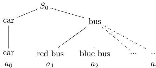
Figure 5: Diagram of the blue Bus/Red Bus environment.
