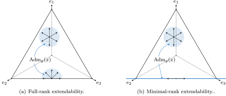
Figure 2. Admissible sets under the Euclidean and Shahshahani metrics. For x \in \mathcal{X}^\circ , we have \text{Adm}_g(x) = \text{TC}_{\mathcal{X}}(x) . For x \in \text{bd}(\mathcal{X}) , we still have \text{Adm}_g(x) = \text{TC}_{\mathcal{X}}(x) in the Euclidean case, but the Shahshahani metric can only be extended to the tangent space \text{Adm}_g(x) = \text{T}_{\mathcal{X}}(x) .
