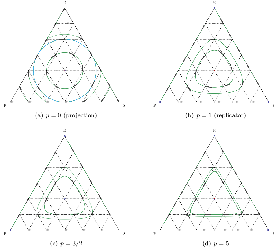
Figure 3. Phase portraits of the p -replicator dynamics in standard Rock-Paper-Scissors. As p \in [0, \infty) increases, the shape of the closed orbits changes from circular to triangular. When p = 0 , solutions enter and leave the boundary of the simplex, but forward solutions exist and are unique. For p \geq 1 , forward and backward solutions exist, are unique, and their support is constant.
