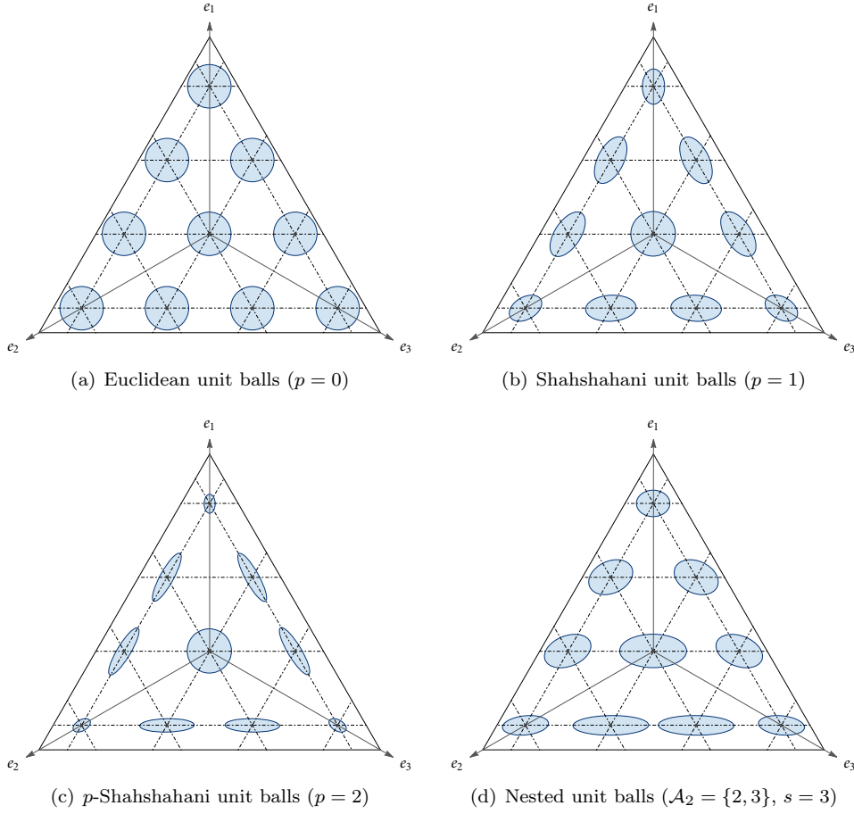
Figure 1. Unit balls on the 3-simplex under the metrics of Examples 3.3–3.6. For each base point x shown, the shaded regions comprise all tangent vectors z based at x that satisfy \|z\|_x^2 \leq 1 .
