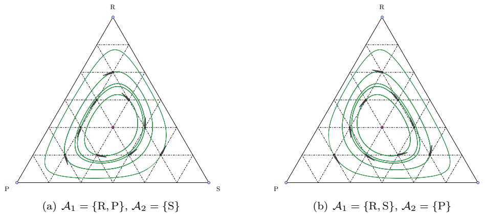
Figure 4. Phase portraits of the nested replicator dynamics in standard Rock-Paper-Scissors with s = 3 for two similarity groupings.
