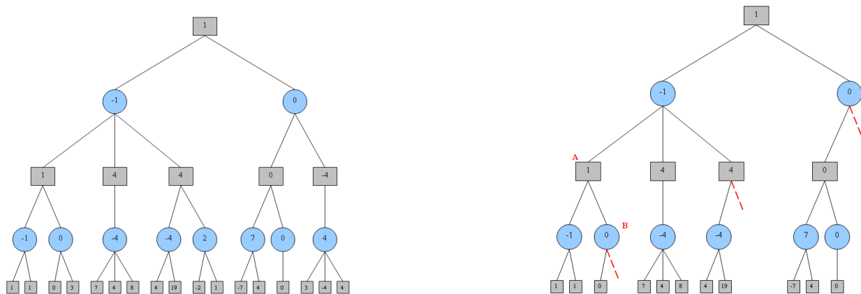
FIG. 1 – Minmax vs alpha-beta
