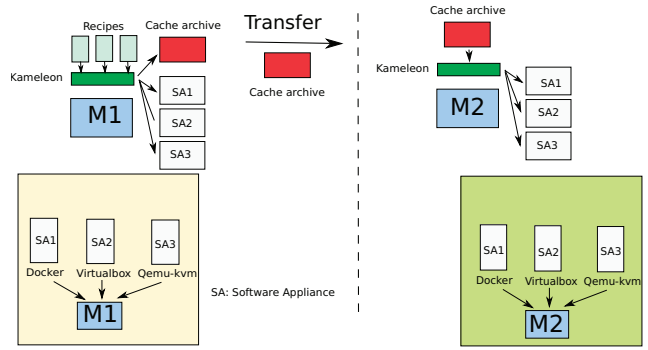
Figure 4: Example of experiment packaging with Kameleon .
